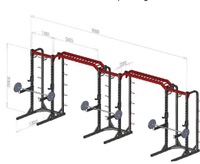
多功能云梯深蹲架 Multi functional cloud ladder squatting frame
